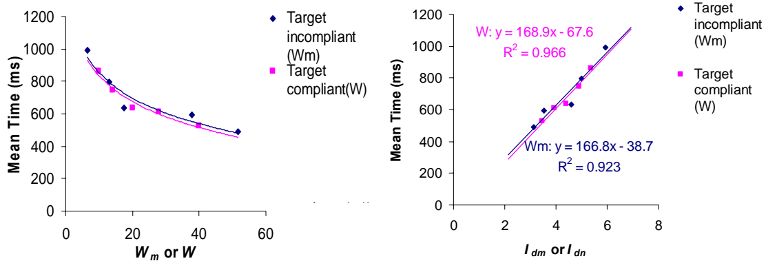
Figure 13. The match between T vs. W_m in the target in compliant scheme and T vs. W in the target compliant scheme (left) and their corresponding Fitts' law regressions (right)
