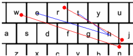
Fig 3. An example of error correction: the user tapped on r-j-n-w but the intended t-h-e is returned.
